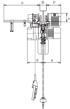
Motor trolley
