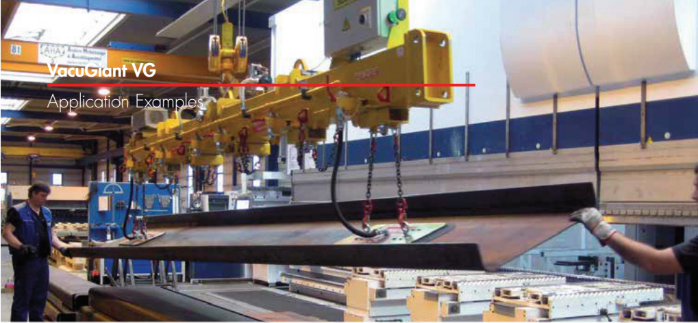
VacuGiant on a bending machine with chain suspension
